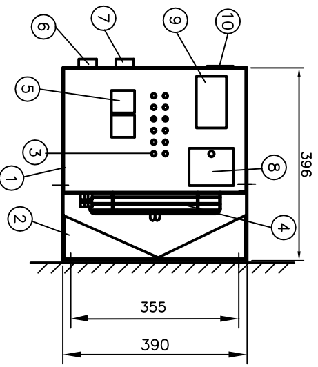
Side view (Service side, without cover)
